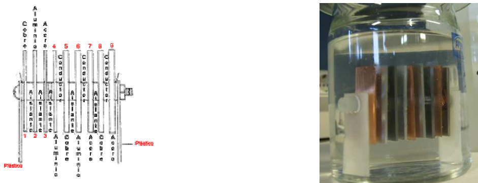
Figure 1: Metal disposition in the corrosion test. In 1 st , 2 nd and 3 rd position we placed aluminium, steel and cupper isolated, avoiding formation of galvanic pairs. In positions 4 and 5, we formed galvanic pairs Al-Cu; in positions 6 and 7 Al-Steel, and in positions 8 and 9 we formed the pair Cu-Steel.
